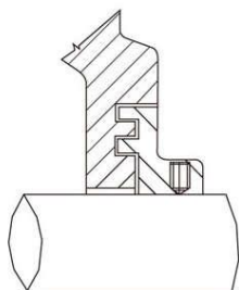
LS SEALING
