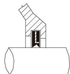
U-LOCK SEALING
