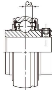
UCX00G Relubricatable type
