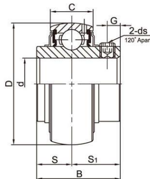
UCX00( Medium Duty) Spherical O.D.
