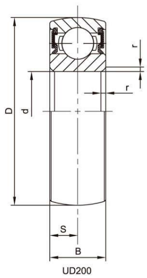
H TYPE SEAL
